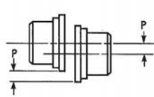
PARALLEL OFFSET MISALIGNMENT
